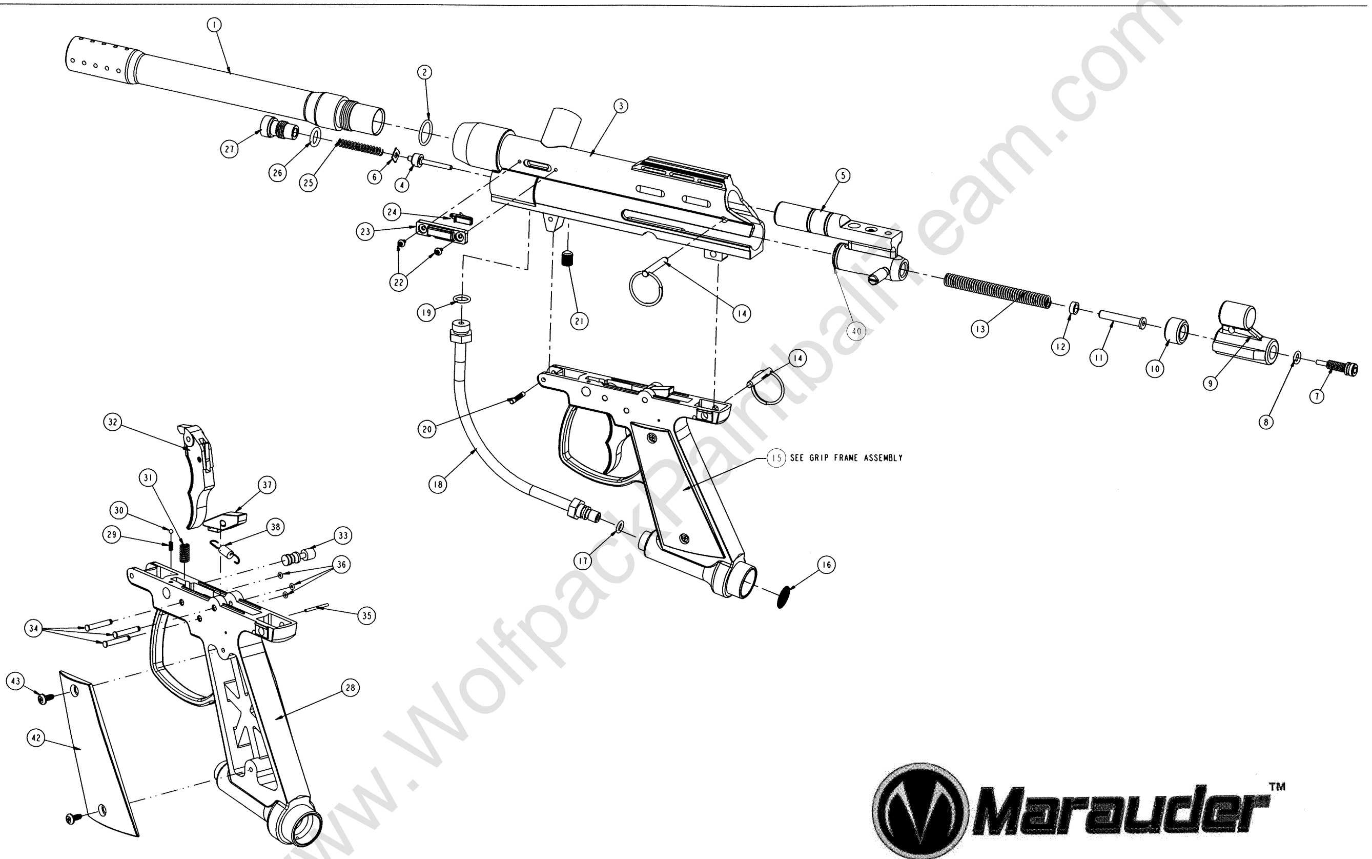
GRIP FRAME ASSEMBLY
